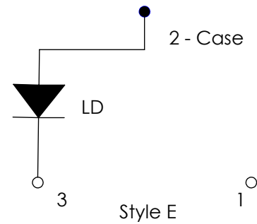
Pin Diagram
