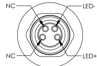
DETAIL A LED OUTPUT CONNECTOR SCALE 2:1
