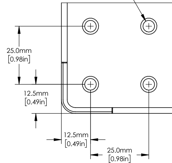
432 X M6 X1.0 TAPPED HOLES THRU TOP SKIN ONLY THREAD DEPTH 6.0mm [0.24in] DETAIL A
