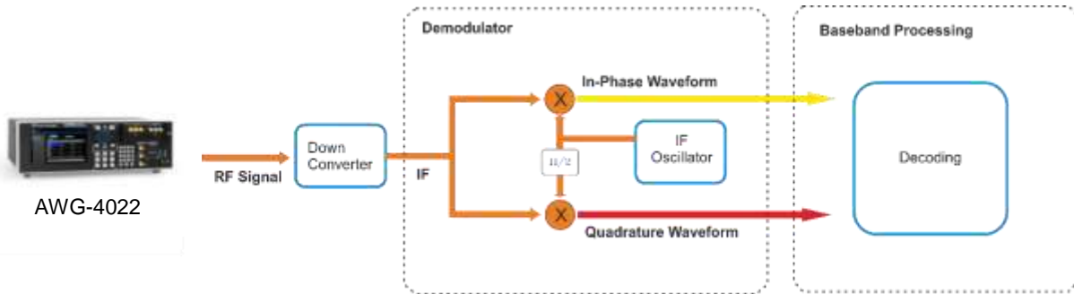
Figure 19: AWG for RF Signals (Receiver test).
