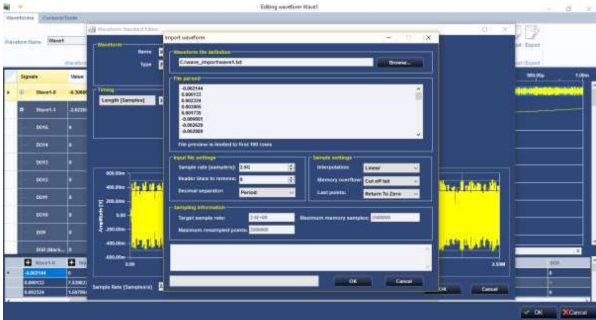
Figure 26: Screen of "Import waveform" page of AWG software.
