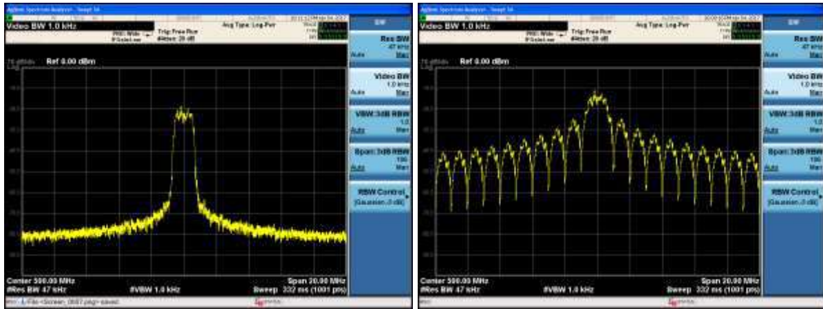
Figure 23: Comparison of 16-QAM spectrum with and without Raised cosine shaping filter.
