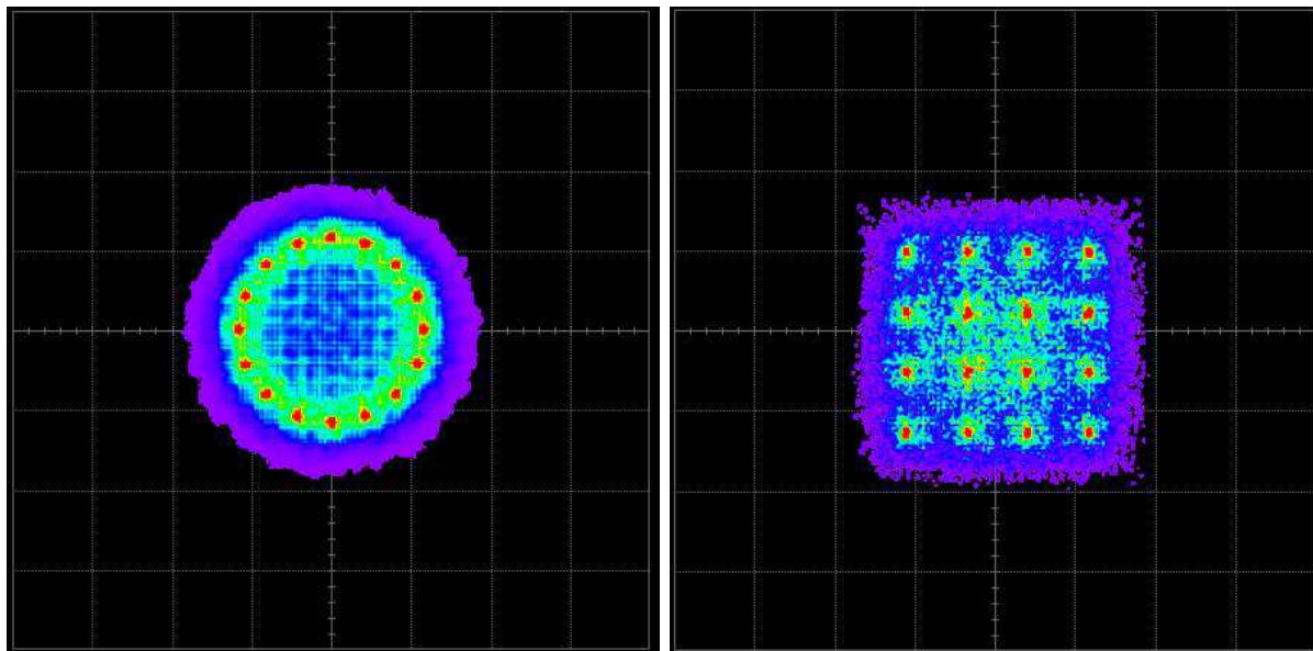
Figure 15: Constellation of 16-PSK and 16-QAM
