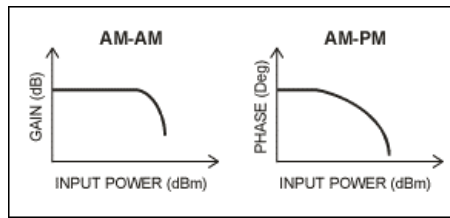
Figure 20: Example of AM/AM and AM/PM graph of an RF power amplifier.
