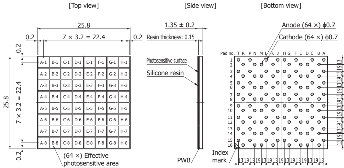
S14161-3050HS-08
