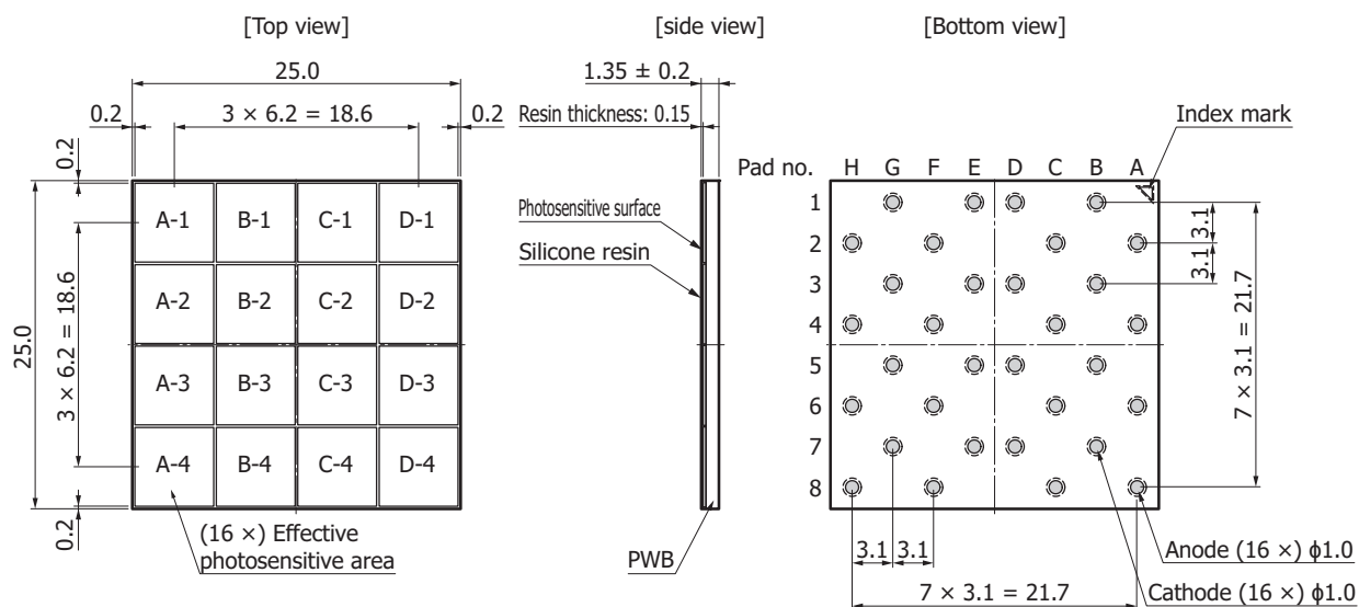
S14161-6050HS-04
