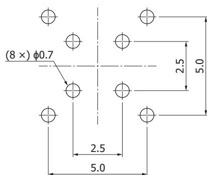
S14160-6050HS
