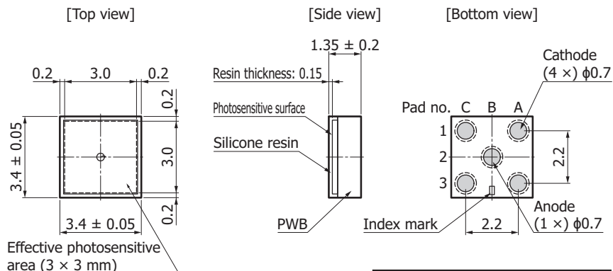
S14160-3050HS
