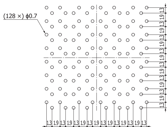
S14161-3050HS-08
