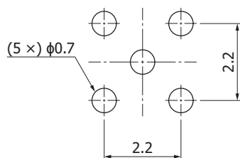
S14160-3050HS
