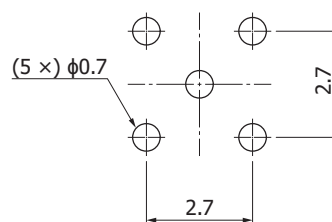
S14160-4050HS
