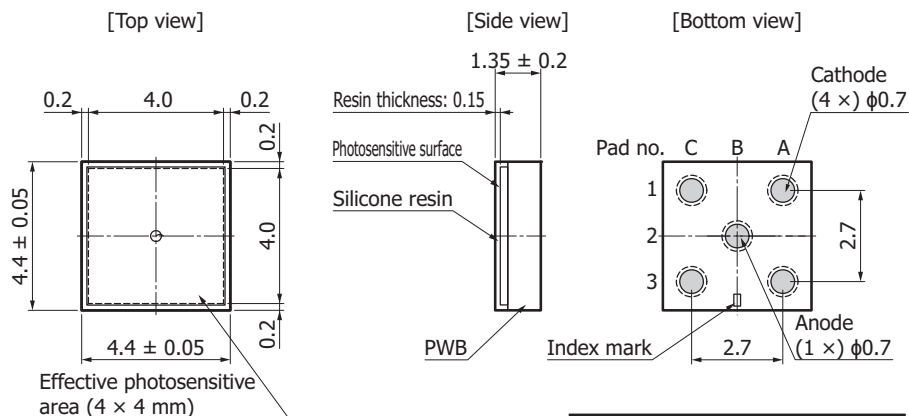
S14160-4050HS
