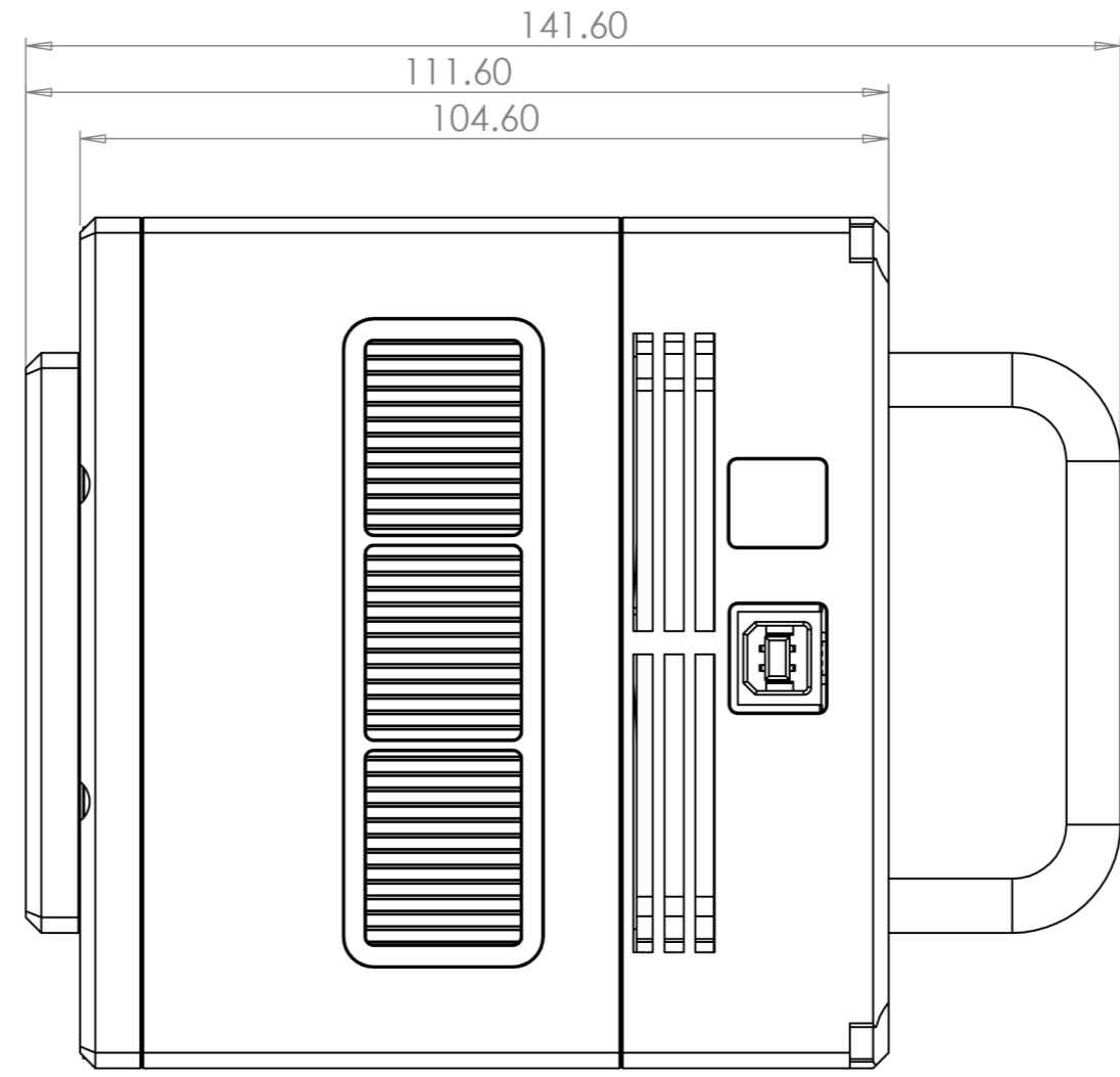
Mechanical drawing Atik 16200
